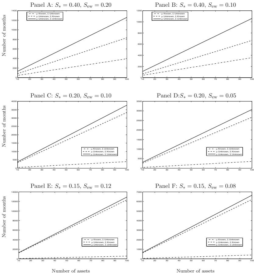
Figure 1 Number of estimation months for mean-variance portfolio to outperform the 1/N benchmark The six panels in this figure show the critical number of estimation months required for the sample-based mean-variance strategy to outperform the 1/N rule on average, as a function of the number of assets, N . Each panel is drawn for different levels of the Sharpe ratios for the ex ante mean-variance portfolio, S_* , and the equally weighted portfolio, S_{ew} . Critical values are computed using the definition in Equation (22). The dashed-dotted line reports the critical value of the estimation window for the case in which the means are known, but the covariances are not. The dashed line refers to the case in which the covariances are known, but the means are not. And the solid line refers to the case in which neither the means nor the covariances are known.
